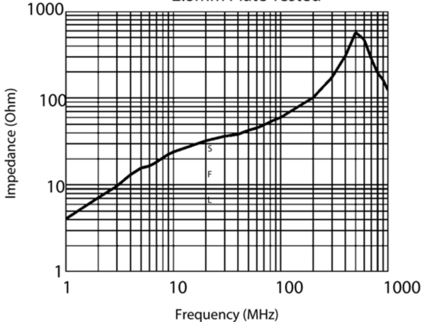
Typical Impedance of KYCON Ferrite D-Sub 2.8mm Plate Tested
