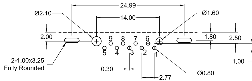
Recommended P.C. Board Layout (Top View)
