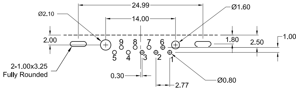
Recommended P.C. Board Layout (Top View)
