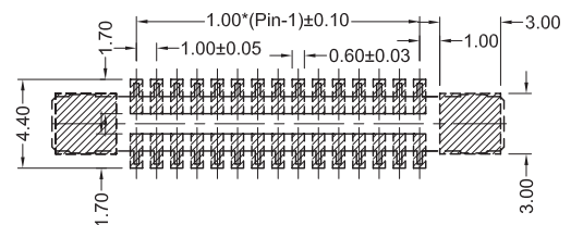
SZVX PCB Layout Reference
